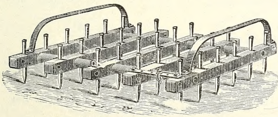
Spike Tooth Harrow—Wood Frame
